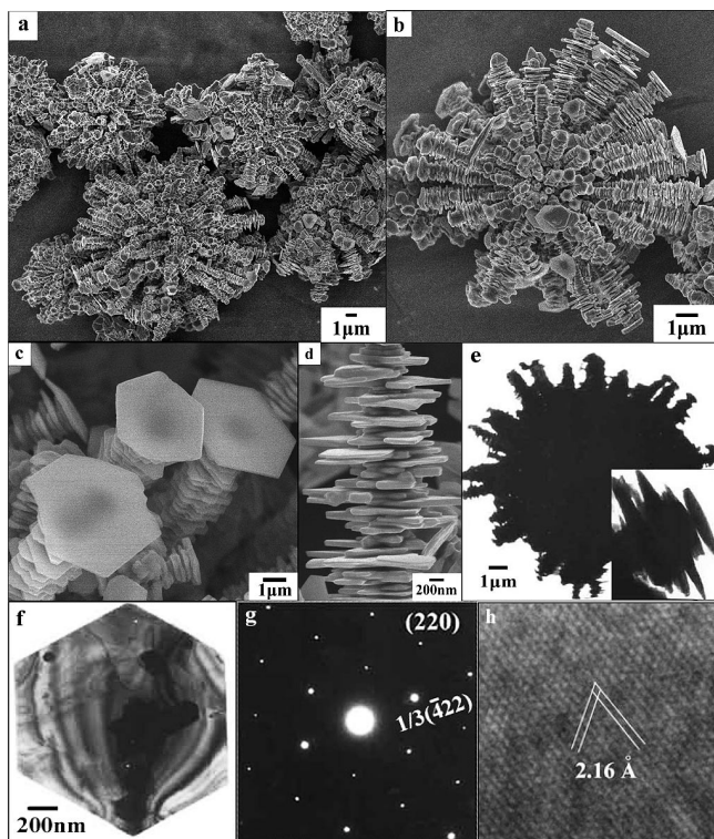
Figure 1. SEM images of the obtained nickel sample: (a) a panoramic image, (b) a typical flowery structure, (c) magnified image of the flowery petals, (d) magnified image of the tops of the petals, (e) TEM image of an individual flower; inset was part of the columnar petal, (f) TEM image of a typical hexagonal platelet unit, (g) the corresponding SAED pattern, (h) HRTEM image of the platelet.
