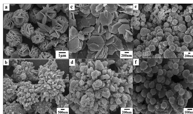
Figure 6. SEM images of the nickel samples prepared from differently shaped \beta\text{-Ni}(\text{OH})_2 precursors: (a) \beta\text{-Ni}(\text{OH})_2 flowers and (b) their reduced product of nickel; (c) hexagonal platelets of \beta\text{-Ni}(\text{OH})_2 and (d) their reduced product of nickel; (e) spherical \beta\text{-Ni}(\text{OH})_2 particles and (f) their reduced product of nickel.
