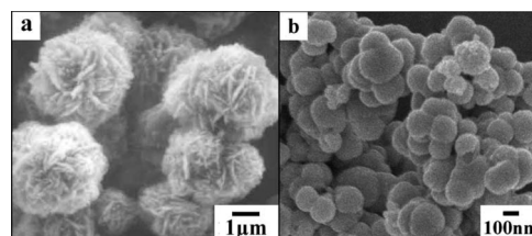
Figure 5. SEM images of the samples prepared at a temperature of (a) 100 °C and (b) 160 °C.
