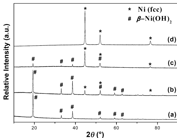
Figure 2. XRD patterns of the product obtained at different reaction stages: (a) 0.5 h, (b) 1.0 h, (c) 3.0 h, (d) 4.0 h.
