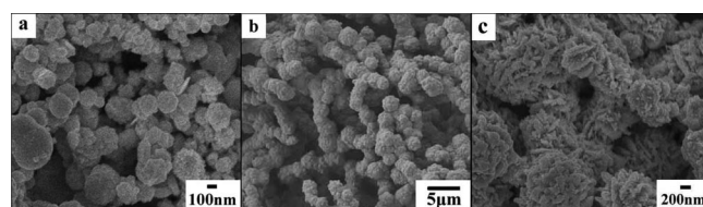
Figure 4. SEM images of the samples prepared in the systems with different molar ratios ( \omega ) of ammonia to hydrazine: (a) \omega = 0 , (b) \omega = 12 , (c) \omega = 18 .
